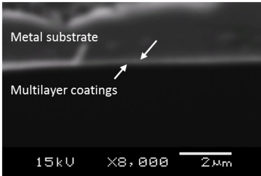
Figure S2. Cross-sectional SEM image of SS-TAPEP 11 surface.
