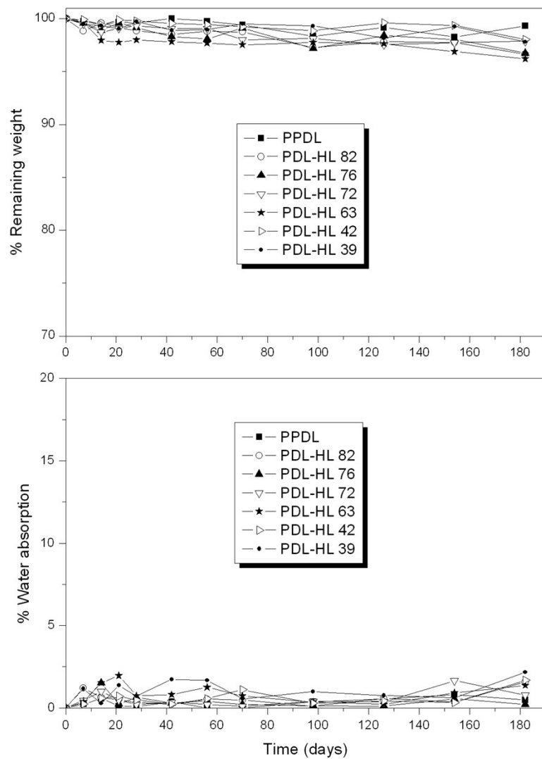
Figure 2. Evolution of the remaining weight and the water absorption of the poly( \omega -pentadecalactone-co- \delta -hexalactone)
