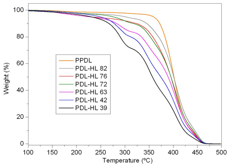
Figure 1. Thermogravimetric (TG) curves of PPDL and the \omega -PDL-co- \delta -HL copolymers.
