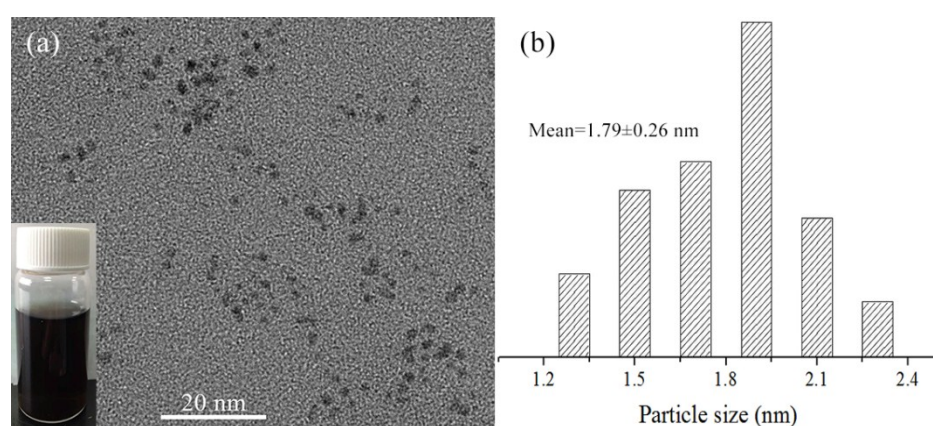
Fig. S1 (a) TEM image (inset is the corresponding solution) and (b) corresponding size distribution histogram for Pt NPs stabilized by PAMAM dendrimers.
