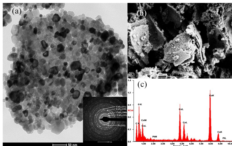
Fig. S2 (a) TEM image of Pt/nano-CeO 2 (inset is the SAED pattern); (b) SEM image of Pt/nano-CeO 2 ; (c) EDX analysis of Pt/nano-CeO 2 .
