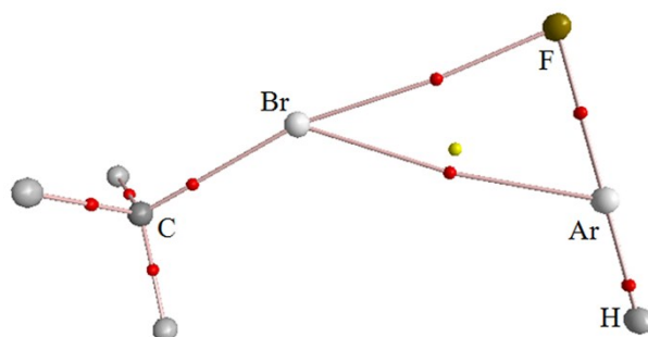
Figure S1. Molecular map of halogen-bonded complex \text{CH}_3\text{Br-HArF}
