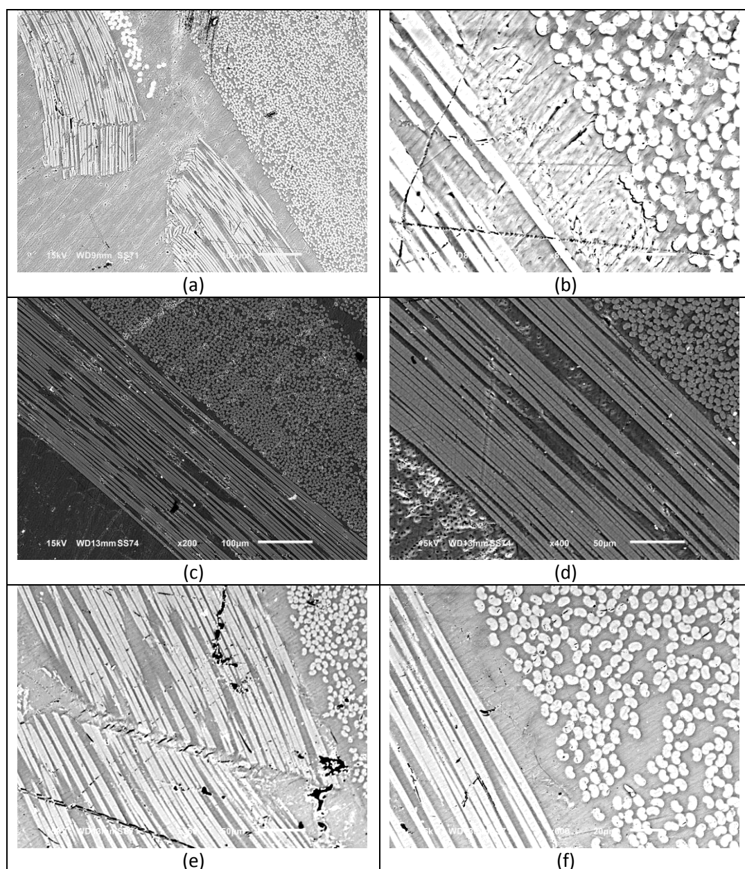
Fig S1. SEM images of cross-sectional area of specimens after flexural failure (a, b) CFRP, (c) CFRP/INT, (d) CFRP/MTX, and (e, f) CFRP/INT+MTX.
