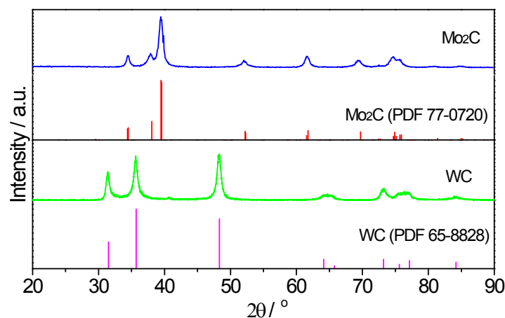
Fig. S1 XRD patterns of \text{Mo}_2\text{C} and WC prepared by TPR method (PDF file references are also included).
