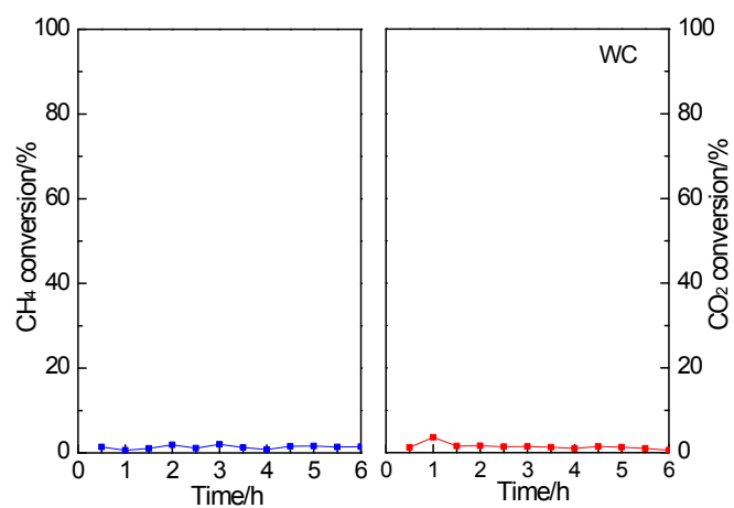
Fig. S3 Lifetime study of WC in DRM (T=800 °C, P=1 atm, CH 4 /CO 2 =1, WHSV=6000 cm 3 g -1 h -1 ).
