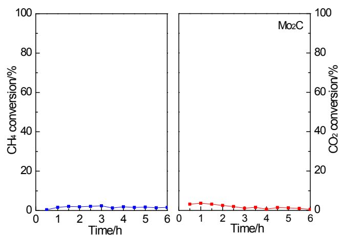
Fig. S2 Lifetime study of \text{Mo}_2\text{C} in DRM ( T=800\text{ }^\circ\text{C} , P=1\text{ atm} , \text{CH}_4/\text{CO}_2=1 , \text{WHSV}=6000\text{ cm}^3\text{ g}^{-1}\text{ h}^{-1} ).
