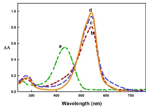
Figure S2. Changes in the absorbance spectra of the studied dye at different pH media
