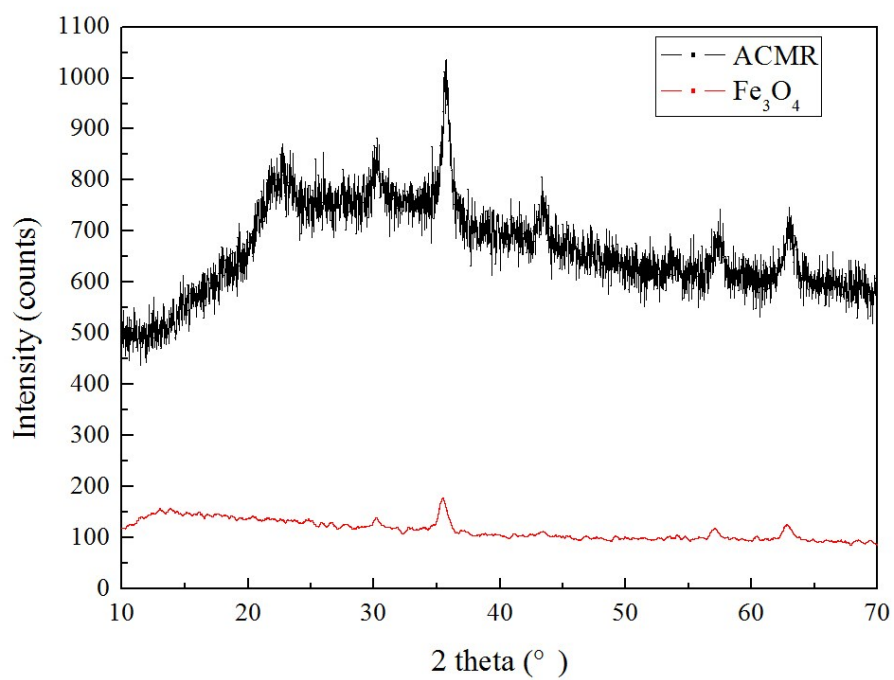
Fig.S1A .The powder X-ray diffraction patterns of ACMR and Fe 3 O 4 .
