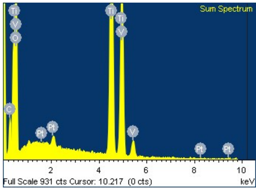
Figure S2 The EDX of the as formed VO 2 coated Ti foil
