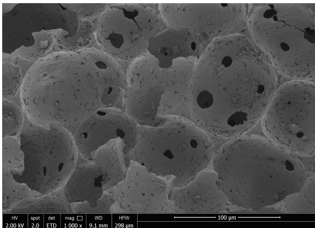
Figure 1 - Cross-section SEM image of P(VDF-TrFE) membrane, 8 % TiO 2 /P(VDF-TrFE) with 3 % NaY.
