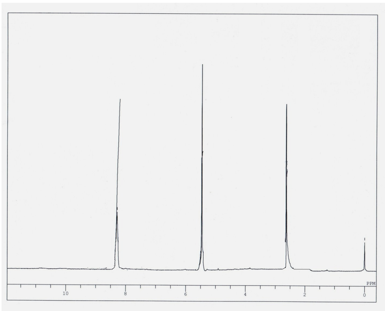
1 H-NMR: 2-(3-amino-5-oxo-4,5-dihydro-1H-pyrazol-1-yl)(p-tolyl)methyl malononitrile (PZ-1)
