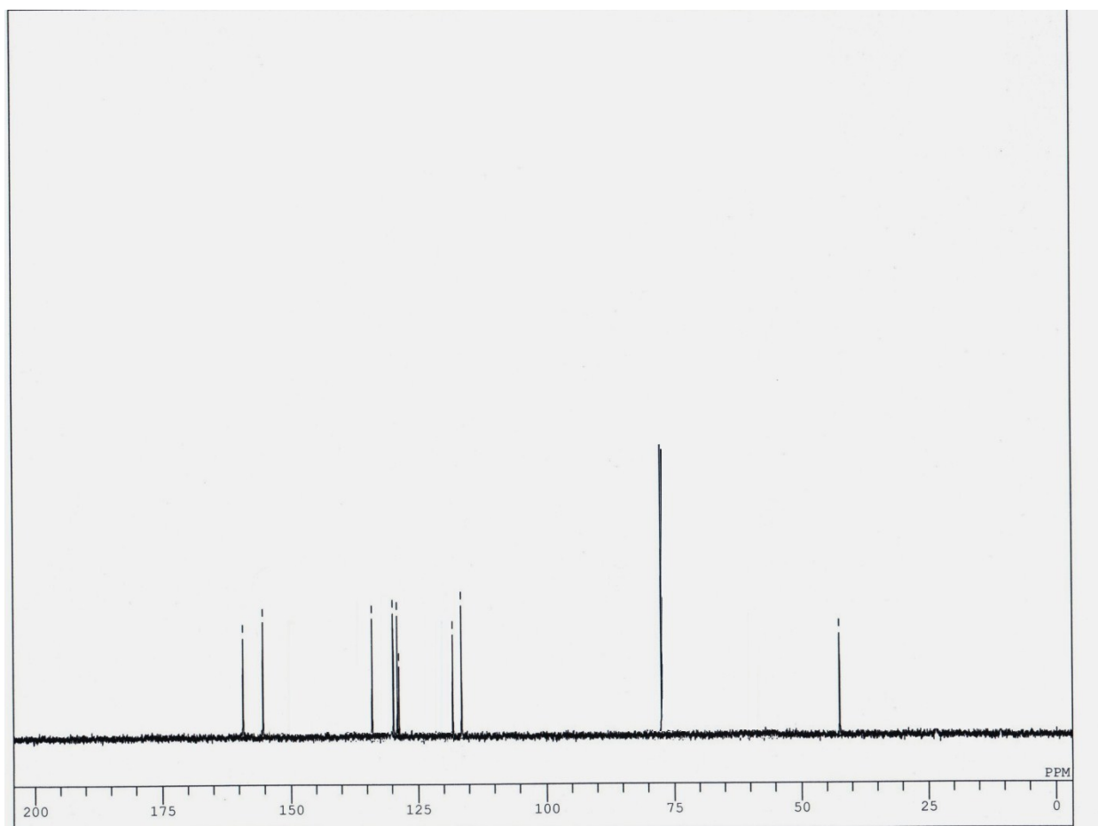
^{13}\text{C} -NMR: 2-(3-amino-5-oxo-4,5-dihydro-1H-pyrazol-1-yl)(phenyl)methylmalononitrile (PZ-2)
