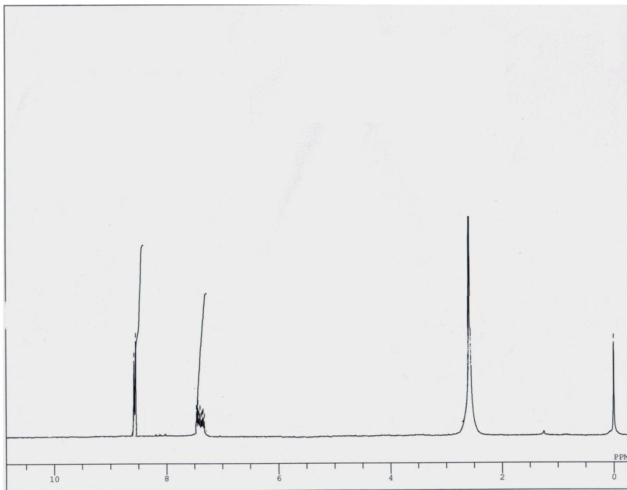
1 H-NMR: 2-(3-amino-5-oxo-4,5-dihydro-1H-pyrazol-1-yl)(phenyl)methylmalononitrile (PZ-2)
