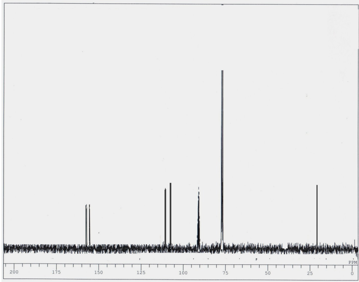
13 C: 2-(3-amino-5-oxo-4,5-dihydro-1H-pyrazol-1-yl)(p-tolyl)methyl malononitrile (PZ-1)
