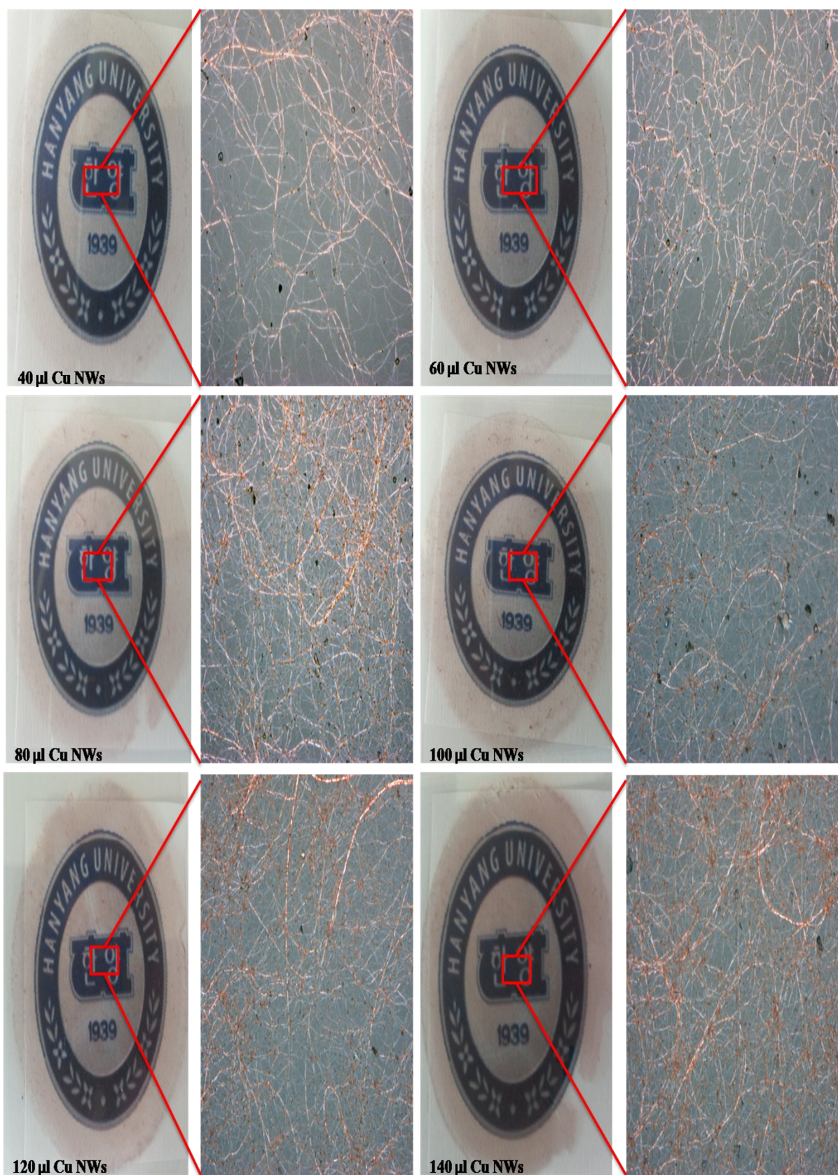
Figure S2: The optical microscopy images of different concentration of Cu NW ink printed on PET substrate.
