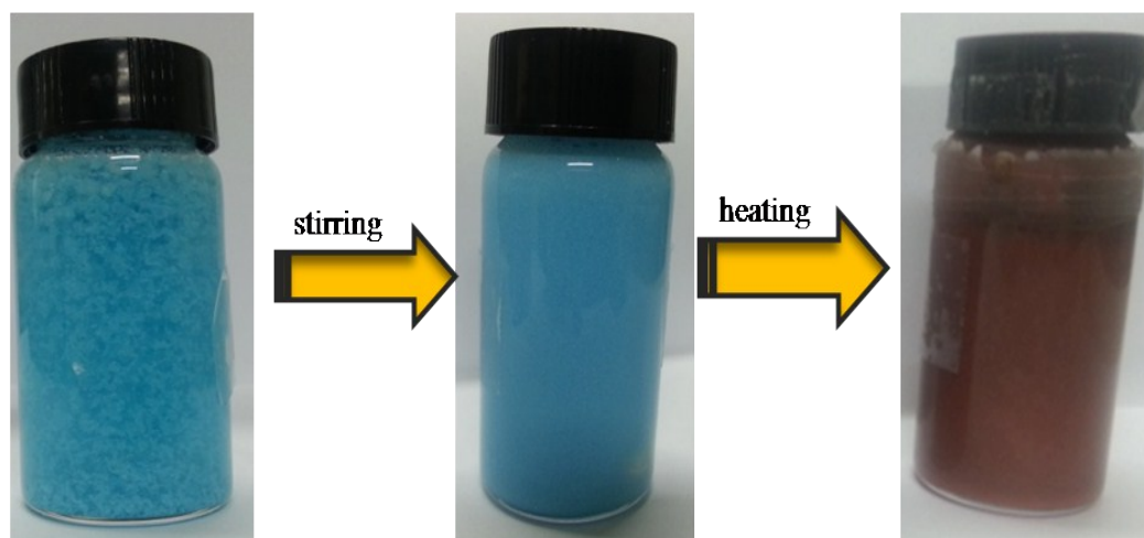
Figure S1: The color changes in the fabrication process of Cu NWs synthesis.
