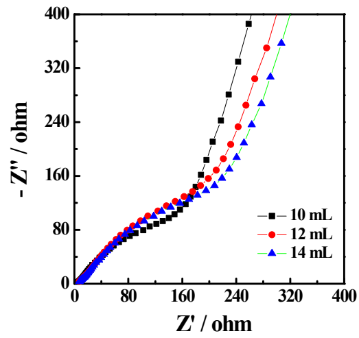
Figure S1. The Nyquist plots of Li/rGO anodes fabricated by different thickness of rGO film.
