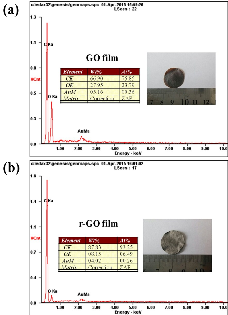
Figure S2. EDS mapping patterns and photographs of (a) GO and (b) rGO films.
