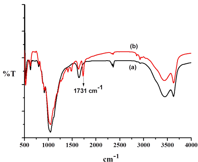
Figure S1: FTIR spectra of a) neat NaMMT and b) NaMMT modified with AETAC.
