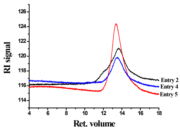
Figure S2: GPC profiles of the fluorinated copolymers prepared via RAFT Pickering miniemulsion polymerization.
