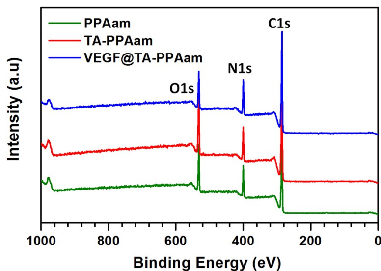
Figure S1. XPS wide-scan survey spectrums of PPAam, TA-PPAam and VEGF@TA-PPAam.
