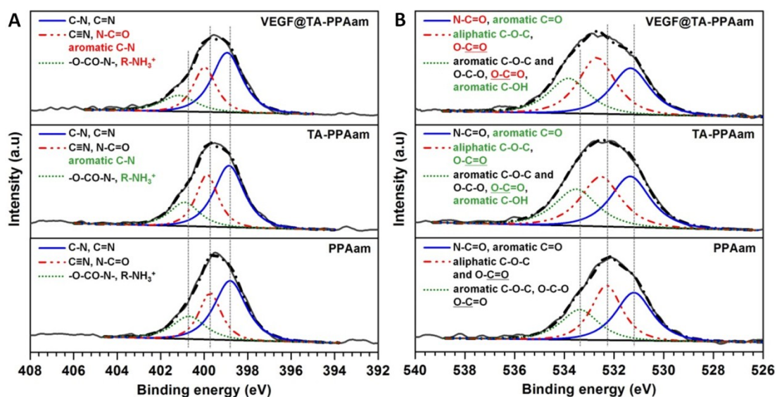
Figure S2. High-resolution spectra of N1s (A) and O1s (B) for PPAam, TA-PPAam and VEGF@TA-PPAam.
