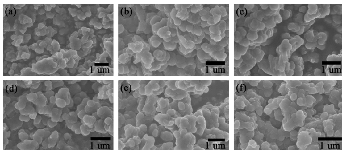
Fig.1. SEM image of the prepared P(1An-1Py) copolymers with different pre-polymerization time: (a) 0 min, (b) 15 min, (c) 30 min, (d) 45 min, (e) 60 min, (f) 120 min.
