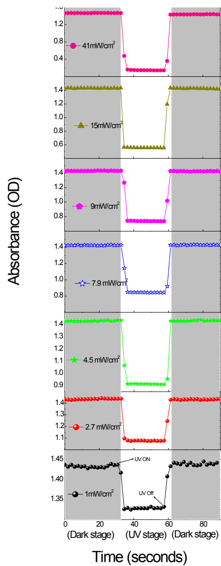
Figure S2 : Showing UV and UV off data of Cu nanoparticles incorporated SD1 with respect to different intensity.
