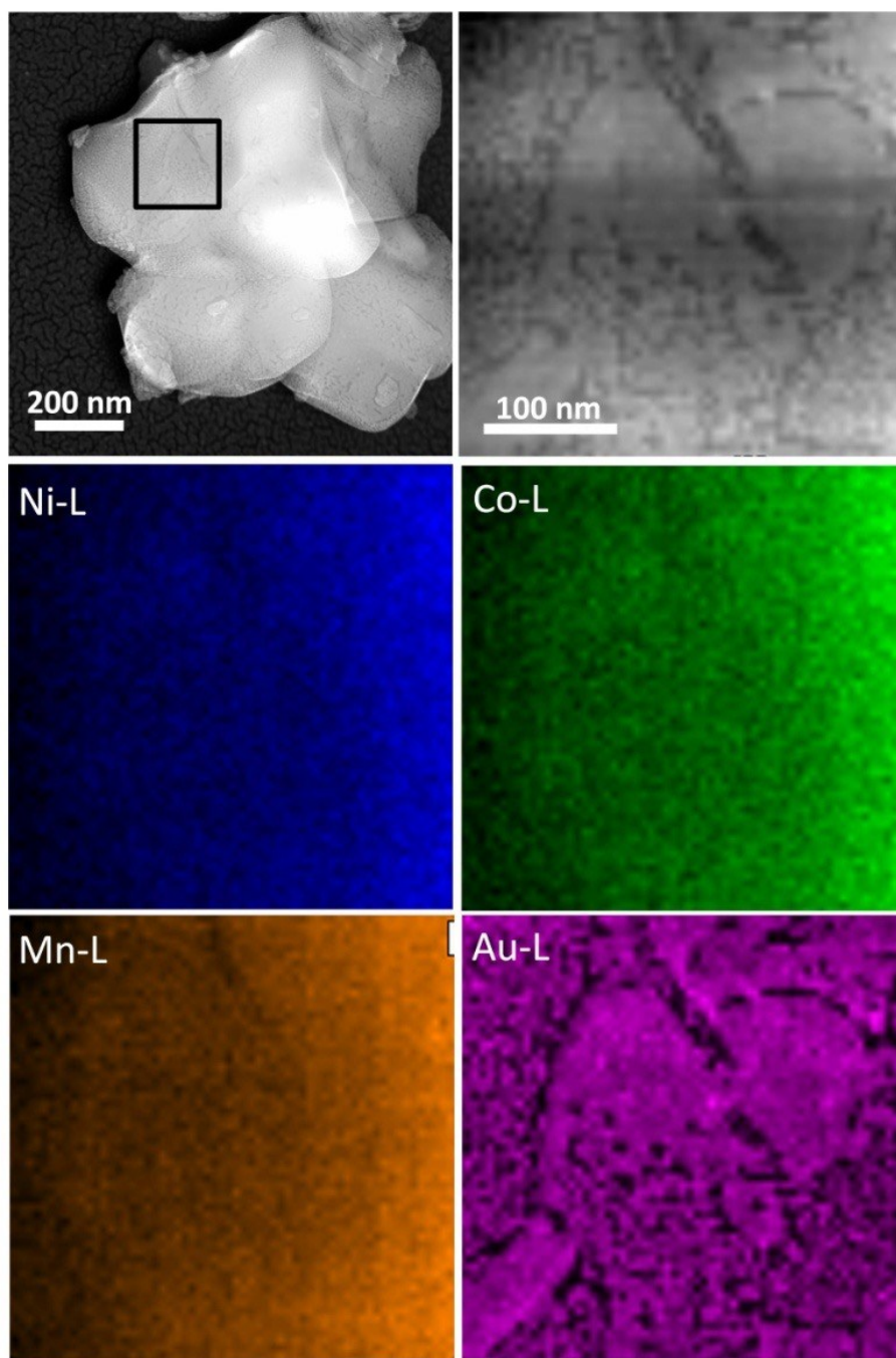
Fig. S2 Elemental mapping of the Au@LMNCO sample by scanning TEM (STEM)
