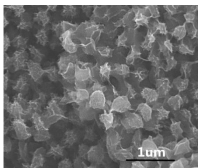
Figure S2 The SEM image of HPCN-850 after 3000 cycles.
