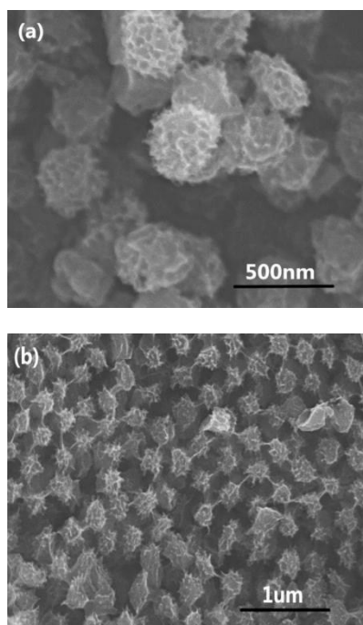
Figure S1 Morphology of as-prepared materials: SEM images of a) HPCNs-750 and b) HPCNs-850.
