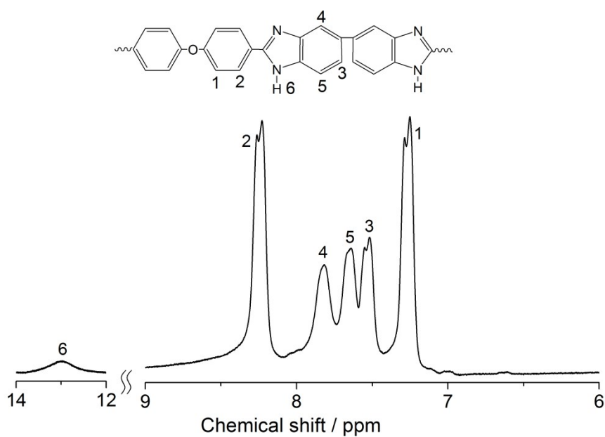
Figure S1. 1 H-NMR spectrum of the synthesized PBI.
