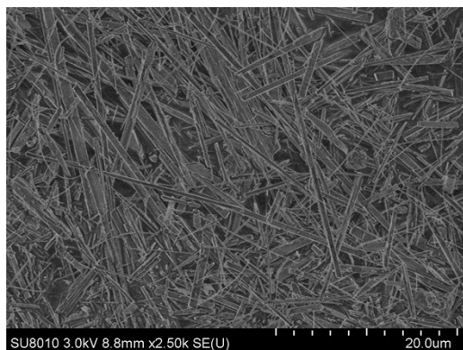
Fig. S1 SEM image of \text{MgF}_2 nanostructures at 950°C showing very thick fibers.
