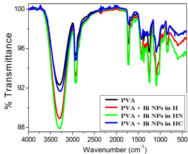
Supplementary Fig.1. FTIR of Bi NPs in PVA at different pH values i.e. Water (H), water +NaOH (HN), and water +HCL (HC).
