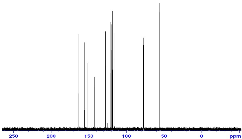
Figure S2. 13 C NMR of N,N-bis(5-chloromethyl-salicylidene)-1,2-phenylenediamine (5-CM-salop)
