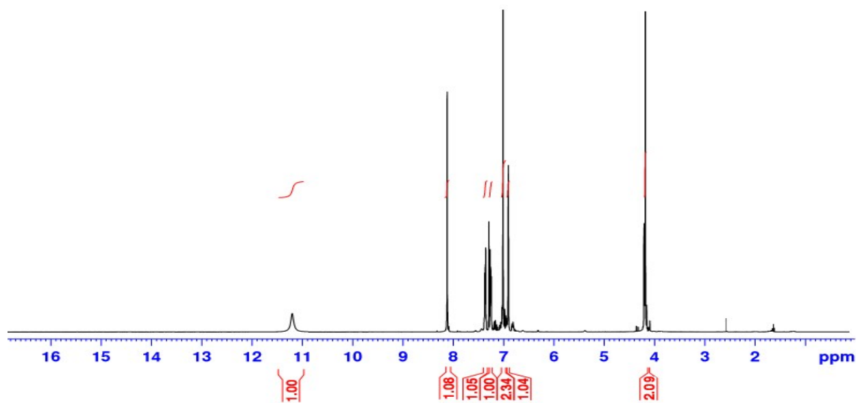
Figure S1. 1 H NMR of N,N-bis(5-chloromethyl-salicylidene)-1,2-phenylenediamine (5-CM-salop)
