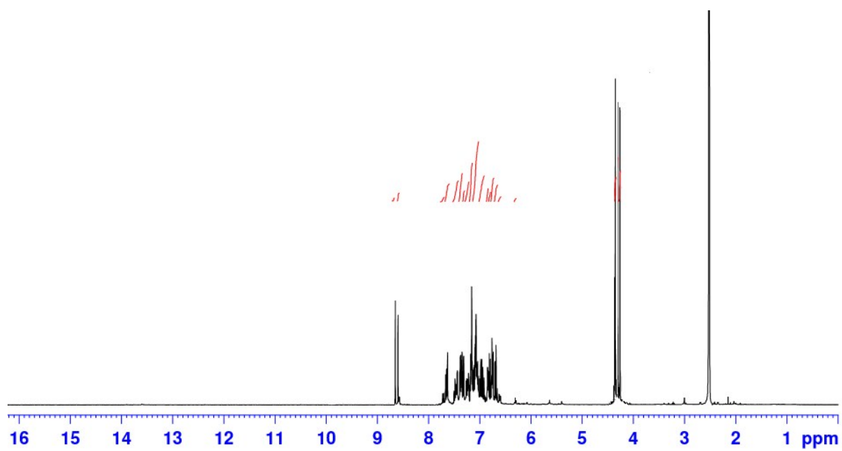
Figure S3. ^1\text{H} NMR of 5-CM-salophMo(O 2 )O complex
