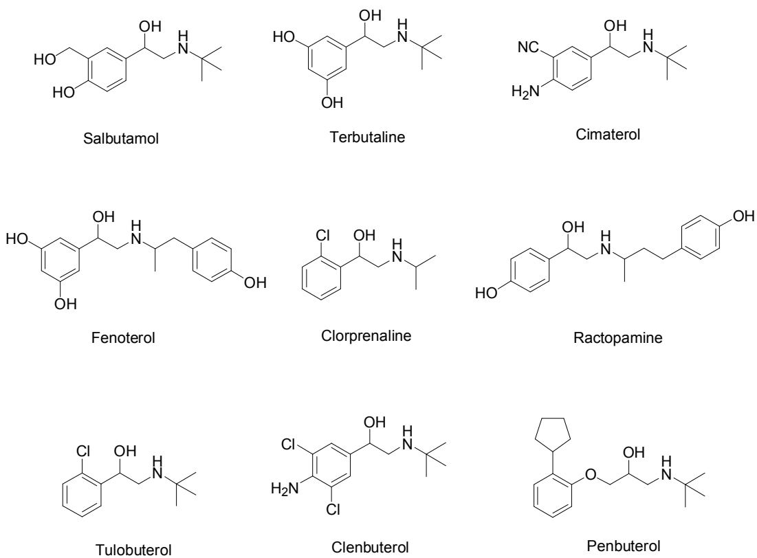
Fig. 1S Chemical structures of nine \beta -agonists
