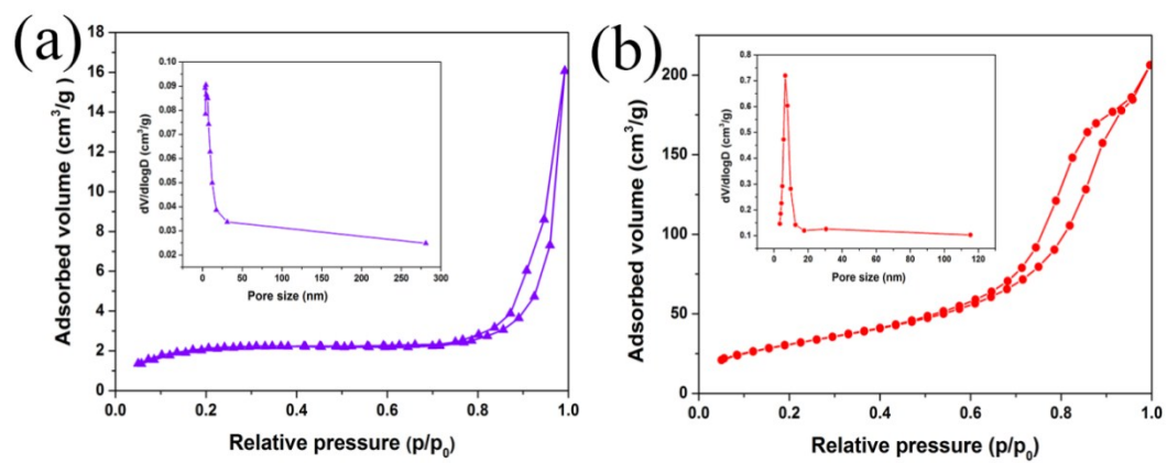
Fig. S3 Nitrogen adsorption-desorption isotherms of CA and 50wt% TiO 2 /CA composite
