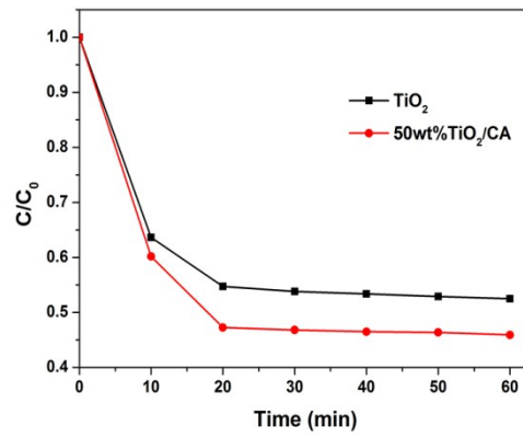
Fig. S6 The adsorption equilibrium curves of \text{TiO}_2 and 50wt% \text{TiO}_2/\text{CA} for CIP over 60 min
