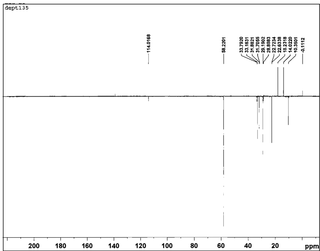
S5: Dept135 ^{13}\text{C} NMR for the isolated product tri(ethoxy)silyl-1-octane.
