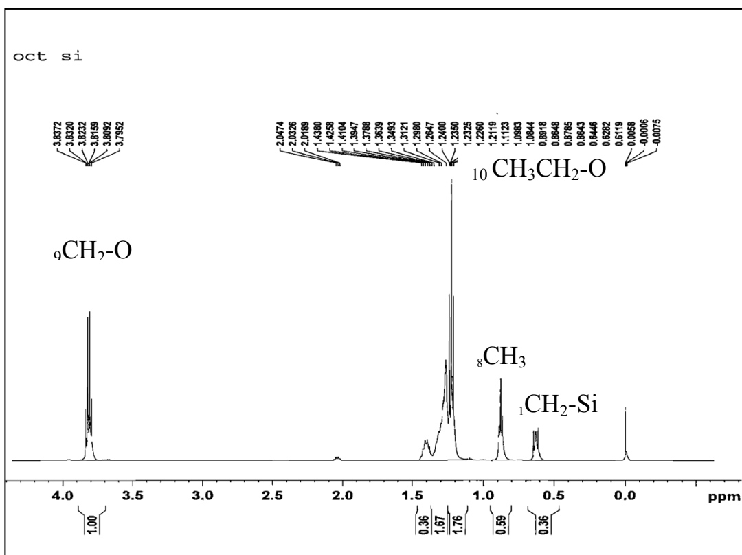
S1: ^1\text{H} NMR for the isolated product tri(ethoxy)silyl-1-octane
