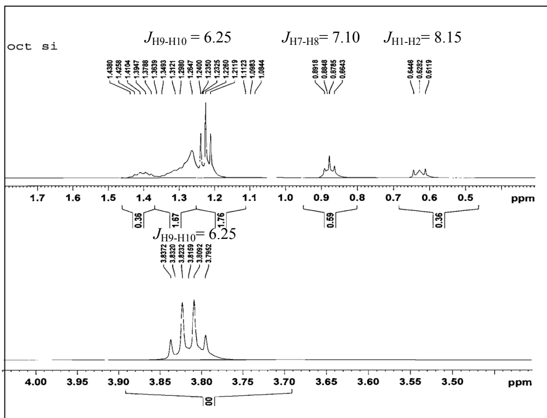
S1: ^1\text{H} NMR for the isolated product tri(ethoxy)silyl-1-octane
