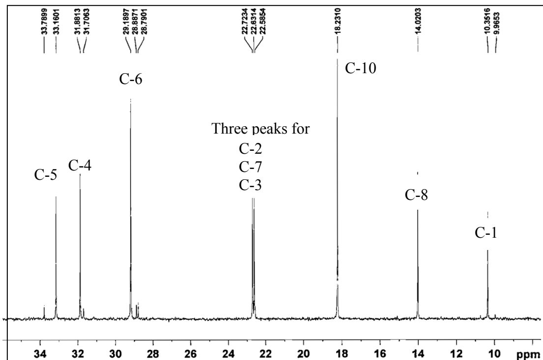
S3: ^{13}\text{C} NMR chart for the isolated product tri(ethoxy)silyl-1-octane.
