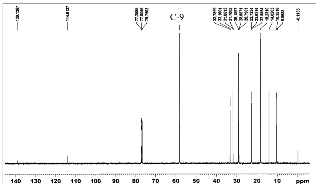
S4: Expanded ^{13}\text{C} NMR chart for the isolated product tri(ethoxy)silyl-1-octane.
