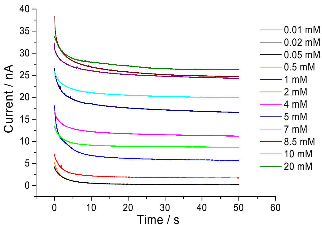
Figure S1. The chronoamperograms performed on solutions with 0.1 M sodium nitrate and different CTAB concentrations.
