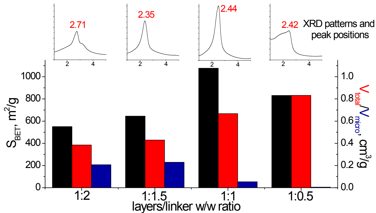
Fig. SI-2. Change of structural and textural properties of hybrid materials obtained using different ratios [layered silica precursor]/[S5 organic precursor].
