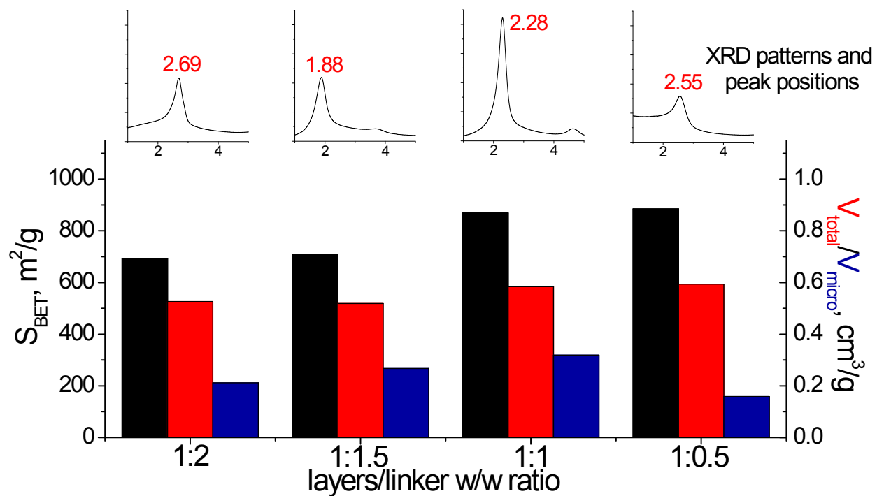
Fig. SI-3. Change of structural and textural properties of hybrid materials obtained using different ratios [layered silica precursor]/[S7 organic precursor].
