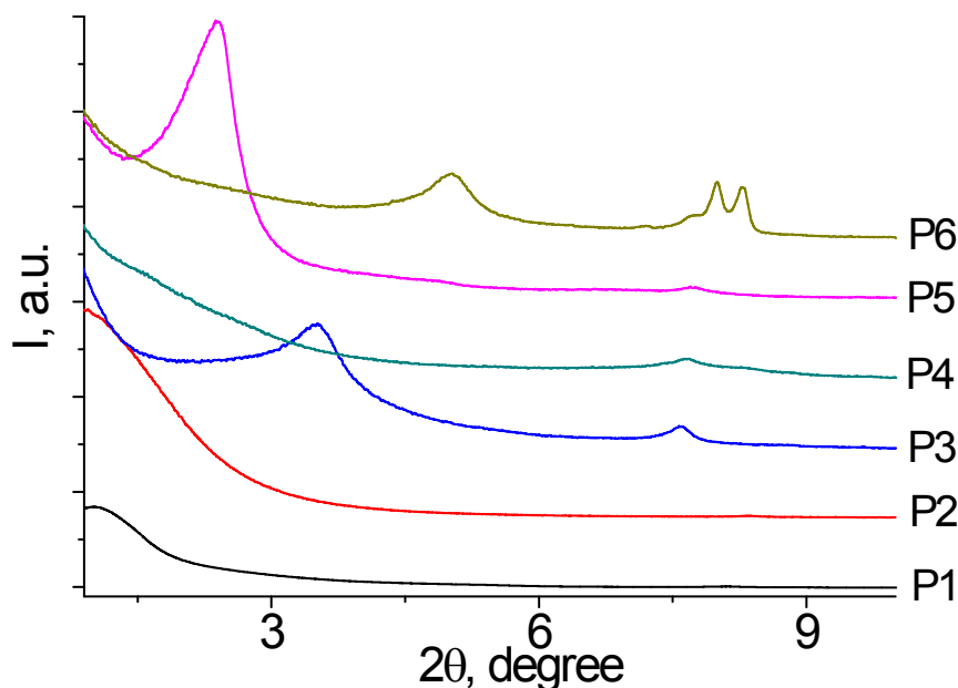
Fig. SI-1. XRD patterns of hybrid materials obtained using different types of polyhedral oligomeric siloxanes.
