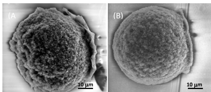
Fig. S1. SEM images of two GO assemblies on a substrate with a trough (A) or a step (B).
