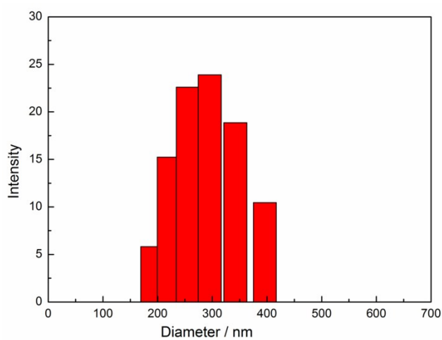
Fig. S2 Size distribution of \text{Fe}_3\text{O}_4@\text{C} SCNCs.
