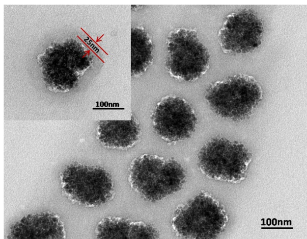
Fig. S1 Representative TEM images of the uniform \text{Fe}_3\text{O}_4@\text{C} SCNCs.
