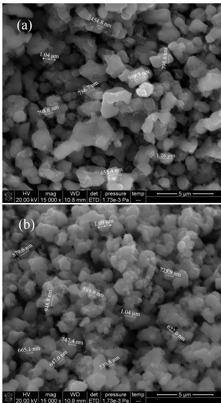
Fig. S1 High- magnification SEM images of (a) LTO-W and (b) LTO-B.
