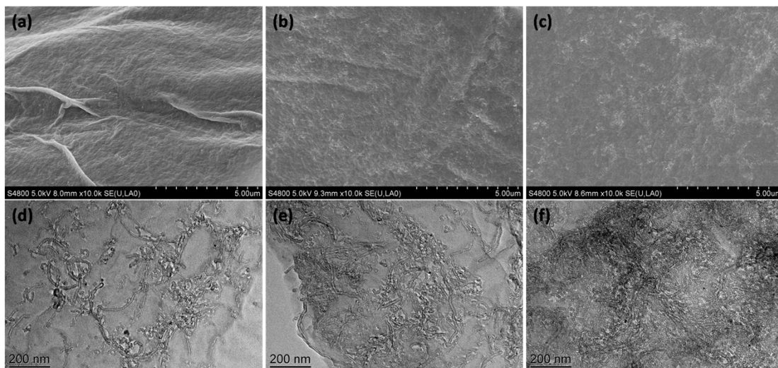
Fig. S1 SEM and TEM images of GNS-1 (a, d), GNS-3 (b, e) and GNS-4 (c, f).
