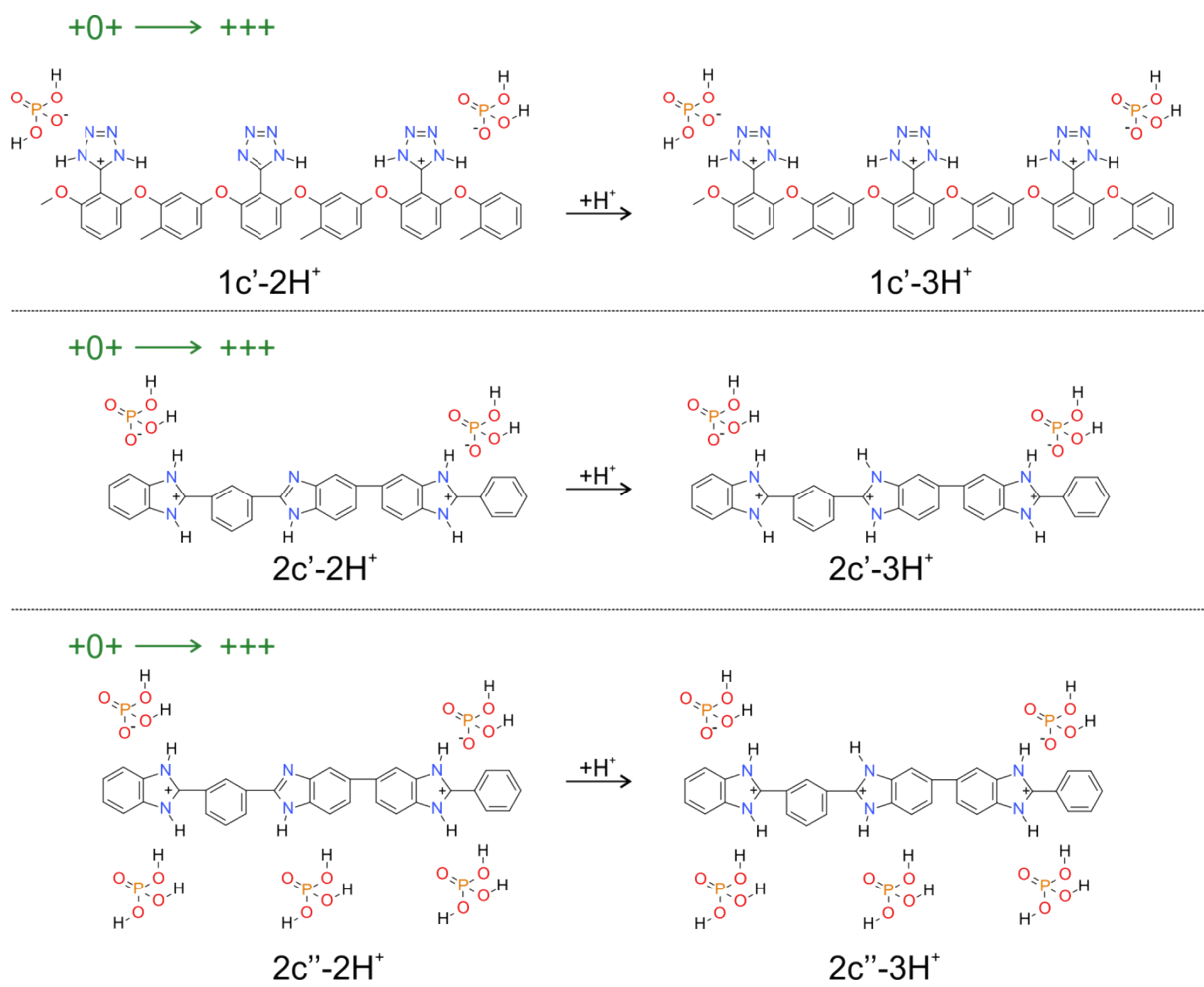
Figure S14. Structure/protonation reactions for systems considered in Table S4 .
