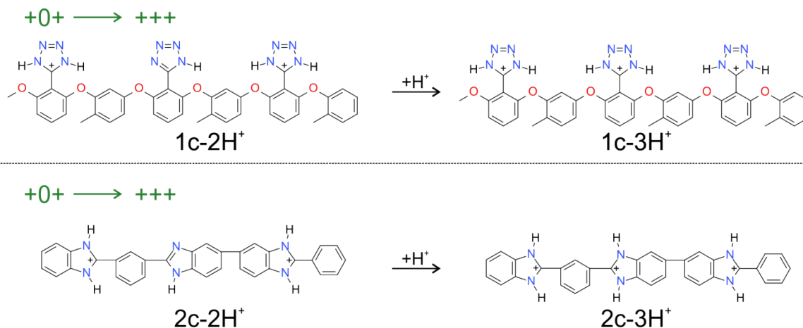
Figure S13. Structures/protonation reaction for systems considered in Table S3 .
