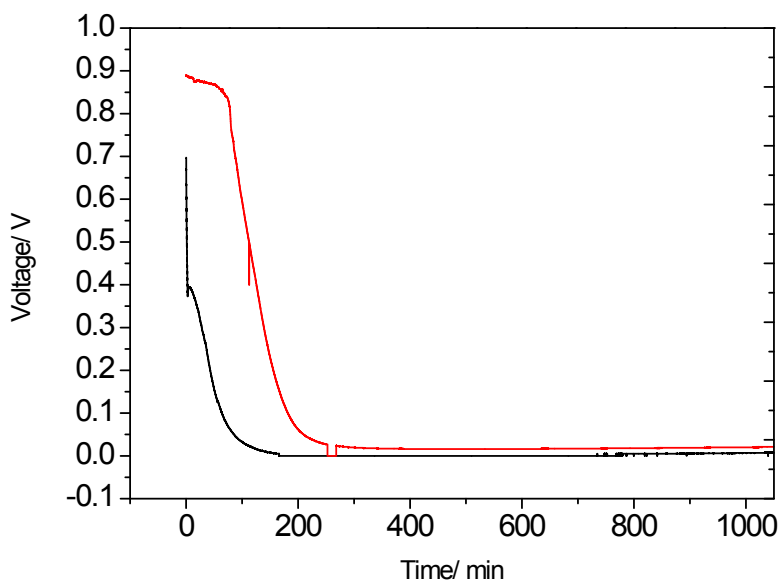
Figure S7: Development of the potential at 0.2 \text{ A}\cdot\text{cm}^{-2} with time for a 40 \mu\text{m} thick TZ-SPEEN membrane ( MEA1 ), doped to a PA uptake of 56% (not dried). Red curve: degradation of potential after the operating temperature of 160 \text{ }^\circ\text{C} was reached. Black curve: potential after shut-down and start-up.
