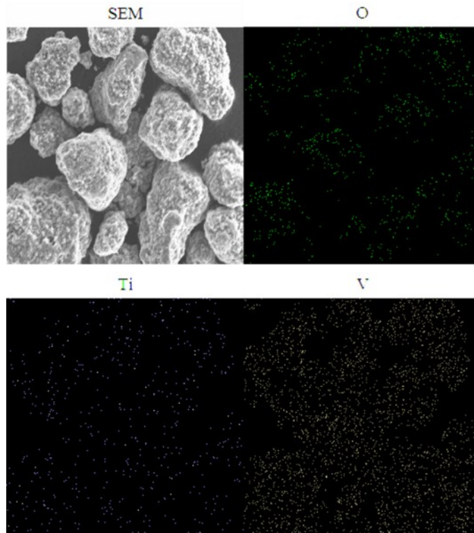
Figure S3 Elemental mapping of \text{TiO}_2\text{-V}_2\text{O}_5\text{-CNT}
