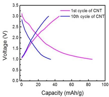
Voltage profile of CNT
