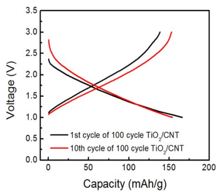
Voltage profile of 100 cycle \text{TiO}_2/\text{CNT}
