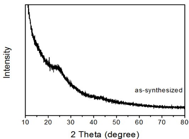
Figure S1 XRD pattern of V_2O_5 -CNT
