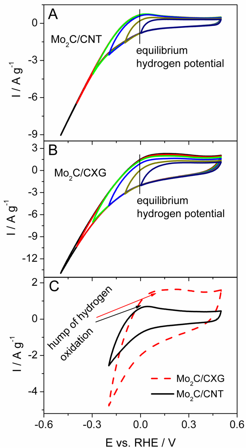
Figure ESI-2. The cyclic voltammograms of Mo 2 C/CNT (A) and Mo 2 C/CXG (B) recorded in 0.1 M HClO 4 with scan rate of 20 mV s -1 with different cut-off potentials.
