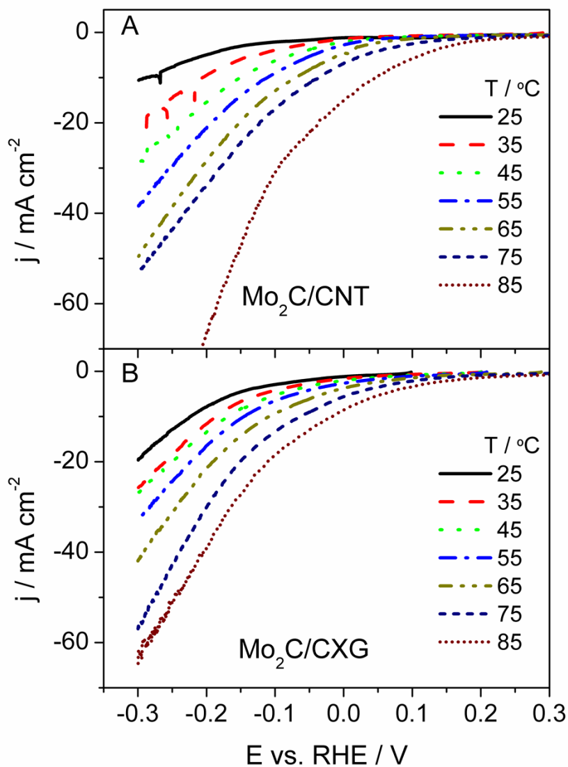
Figure ESI-1. Polarisation curves of \text{Mo}_2\text{C/CNT} (A) and \text{Mo}_2\text{C/CXG} (B) in 0.1 M \text{HClO}_4 in the 25–85 °C range.
