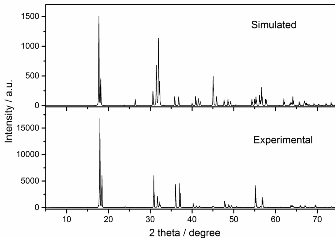
Figure S1. XRD pattern of \text{Ca}_2\text{PbO}_4 experimental sample comparing with simulated data from single-crystal
