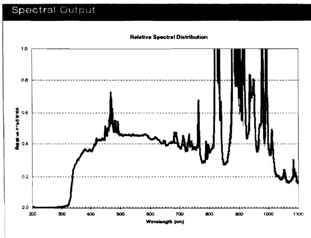
Figure S2. The relative spectral distribution of the 300 W Xe lamp.
