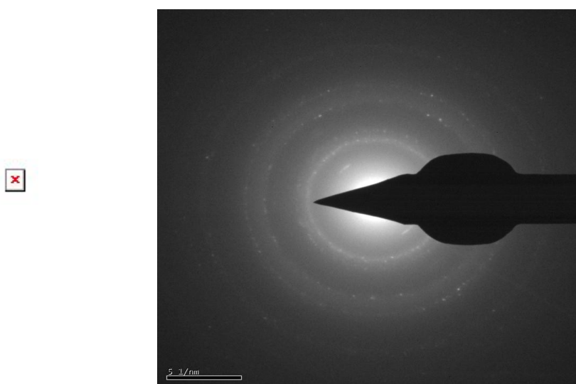
Figure S2: SAED of Co/Ni decorated SWCNT
