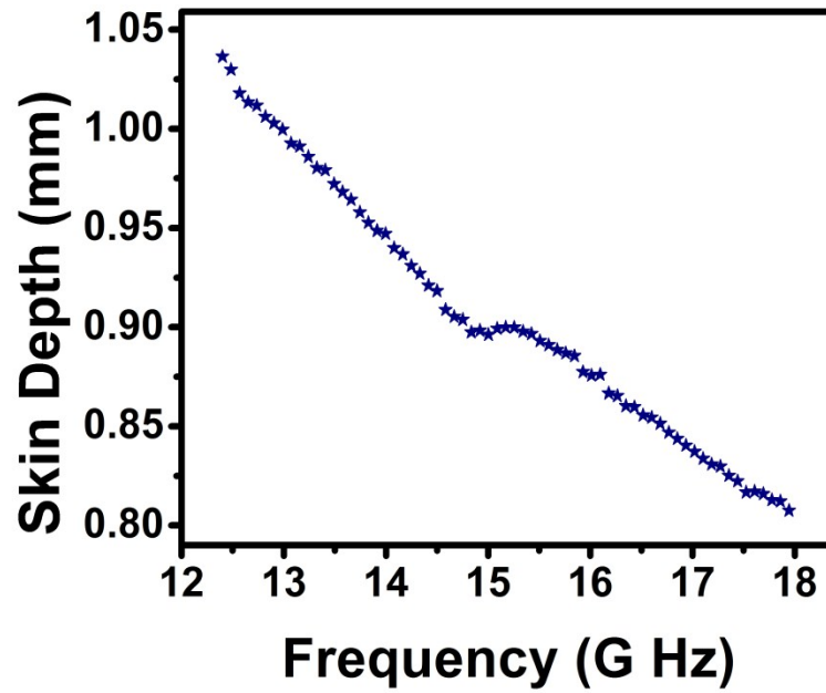
Figure S4: Variation of skin depth with frequency
