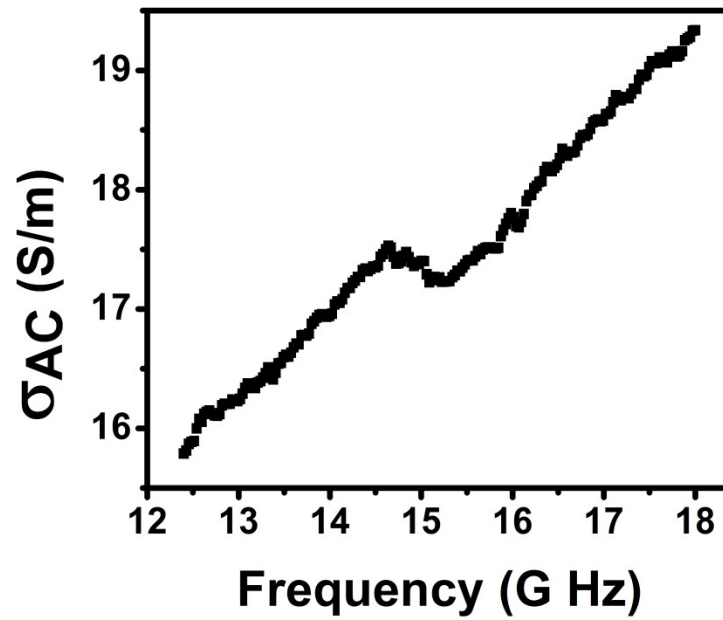
Figure S3: Variation of electrical conductivity with frequency
