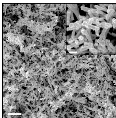
Figure S2 SEM image of a CNT forest coated with 30 nm tungsten. The scale bars are 1 \mu\text{m} and 200 nm for the figure and inset, respectively.
