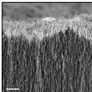
Figure S1 Cross-section image of a CNT forest coated with 150 nm tungsten. The scale bar is 5 \mu\text{m} .
