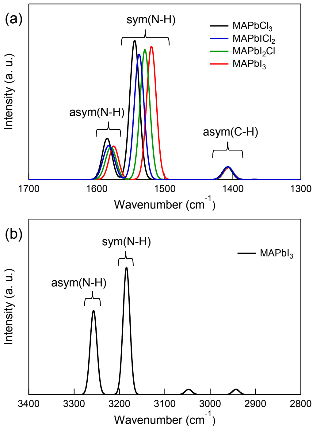
Figure S1. The simulated absorption spectra of MAPbCl 3 , MAPbICl 2 , MAPbI 2 Cl, and MAPbI 3 at low frequency region (a) and simulated absorption spectra of MAPbI 3 at high frequency region.
