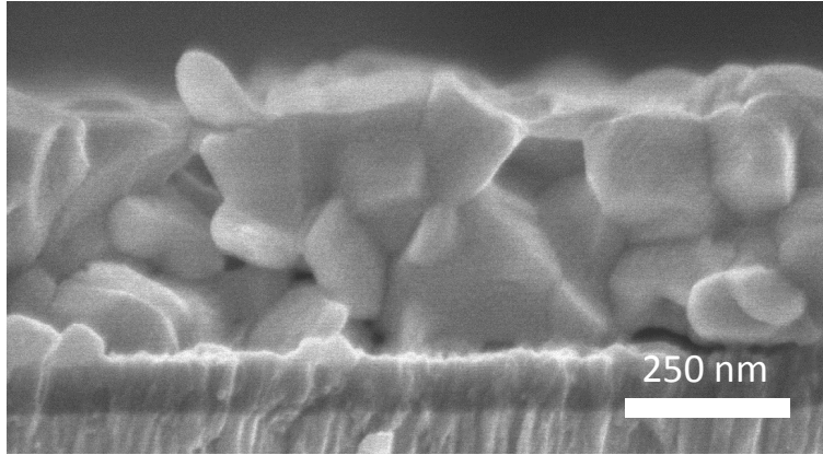
Figure S2. Cross-sectional SEM images of the TI perovskite layer annealed for 15 minutes.
