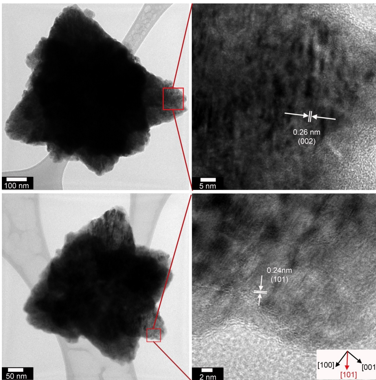
Fig. S1 High resolution TEM of precipitated single flower-shaped ZnO particle (ZN-8g) confirming the c-axis orientation of primary nanoparticles.
