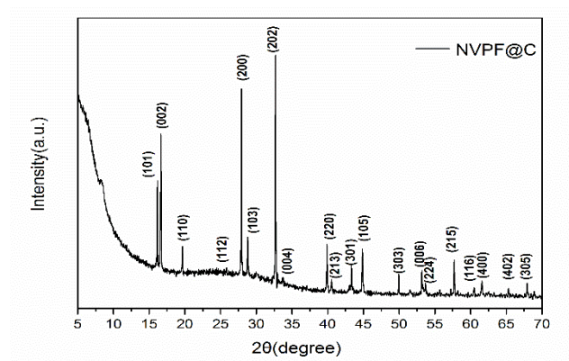
Figure S3. XRD patterns of NVPF@C.
