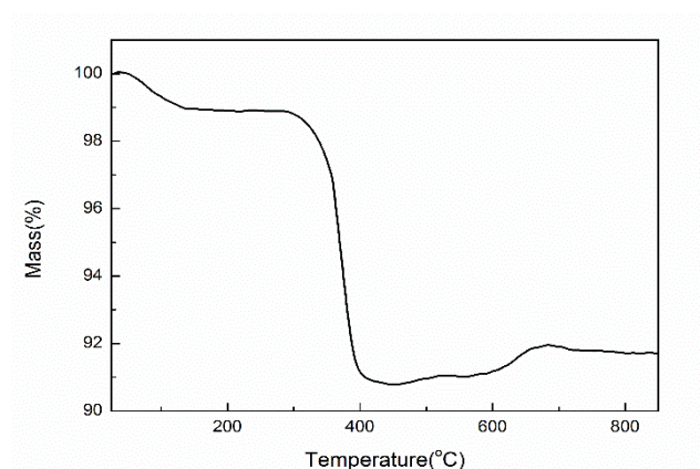
Figure S1. TG curves of NVPF@C/G sample (The TG (STA409PC) result was under a heating rate of 10°C/min and the air atmosphere flowing rate of 25 mL/min.)
