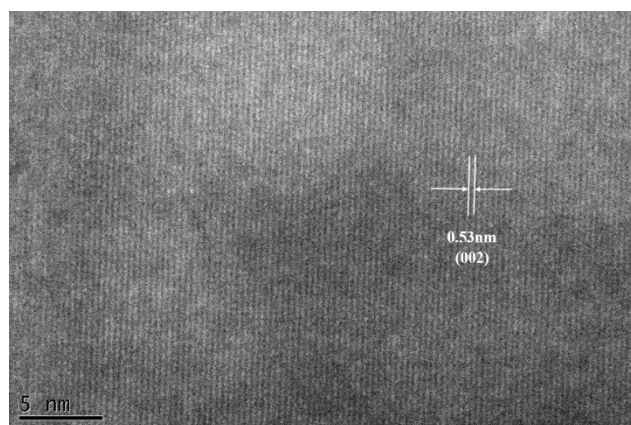
Figure S2. HRTEM image of NVPF@C/G
