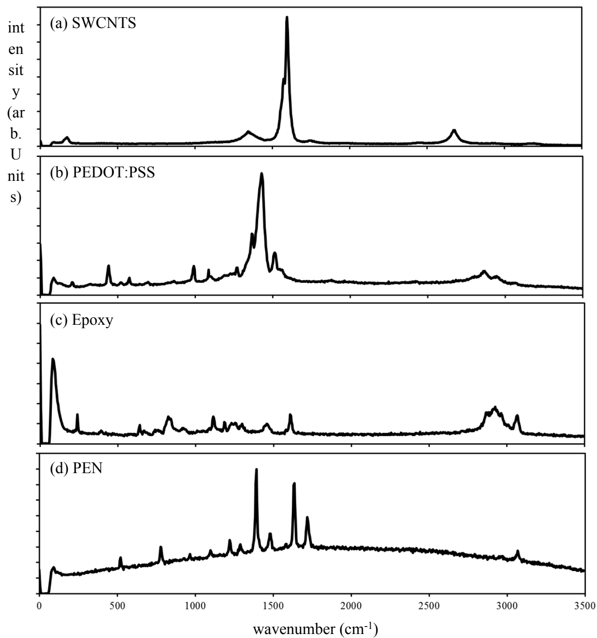
Figure 1: Control Raman spectra of individual components of AgNW:SWCNT:PEDOT:PSS electrodes. (a) SWCNTs, (b) PEDOT:PSS, (c) Epoxy and (d) PEN. Raman spectra for each component matches literature.
