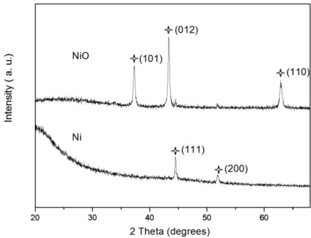
Fig.S1 XRD patterns of the obtained NiO and Ni NFs.
