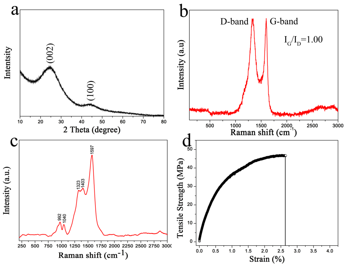
Fig. S2. (a-b) The XRD pattern and Raman spectra of HDC. (c) Raman spectra of HDC@NiCo 2 O 4 @PPy composites. (d) Typical stress-strain curves of the fiber-shaped SCs.
