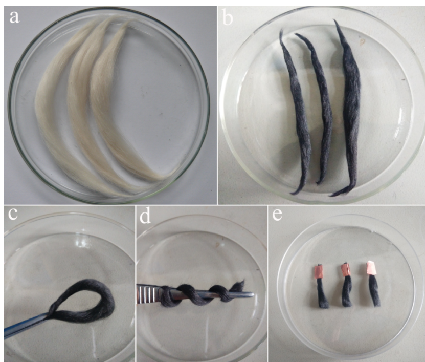
Fig. S1. (a-b) Photographs of the original hemp fibers and HDC. (c-e) Photographs of the flexible HDC.
