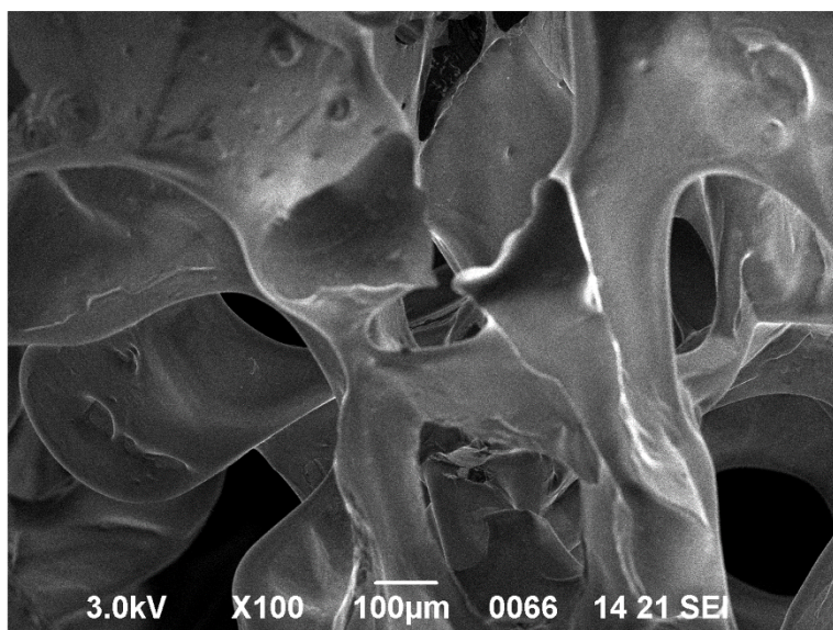
Figure S2 SEM image of porous PDMS with the size of GMps equal to 620 \pm 100 \mu\text{m}
