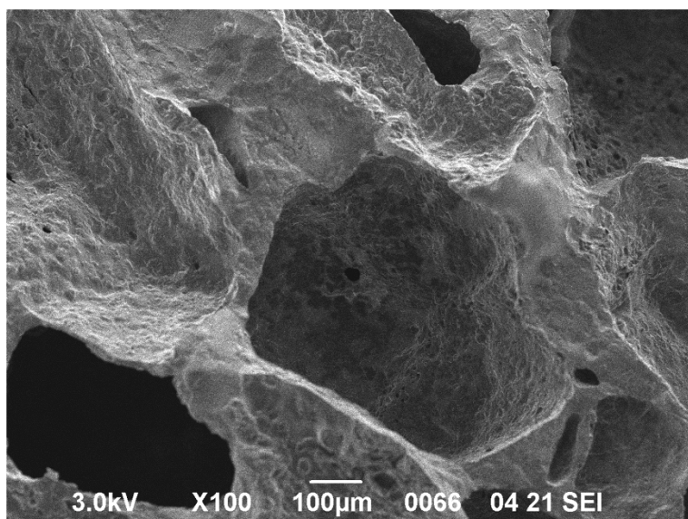
Figure S1 SEM image of porous PDMS-MWNTs with the size of GMps equal to 620 \pm 100 \mu\text{m}
