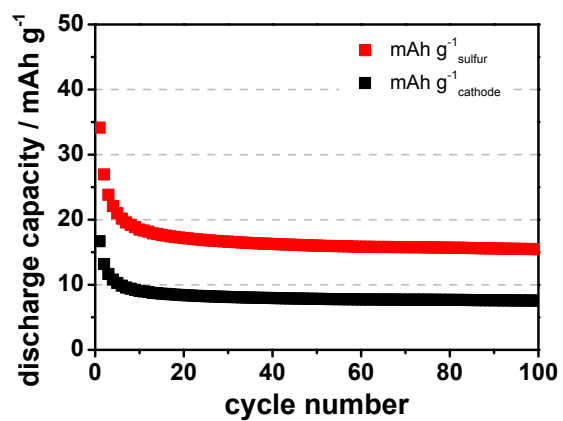
Figure S1 Discharge capacity of cathodes from pristine \text{Li}_2\text{SO}_4 \cdot \text{H}_2\text{O} reduced at 900 °C.
