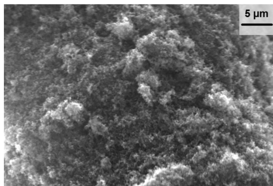
Figure S2 SEM image of 84 h ball milled \text{Li}_2\text{SO}_4 \cdot \text{H}_2\text{O}
