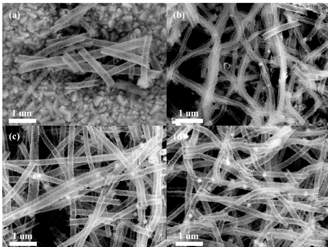
Fig. S2. FE-SEM (back-scattering mode) images of (a) AS0, (b) AS1, (c) AS2 and (d) AS3.
