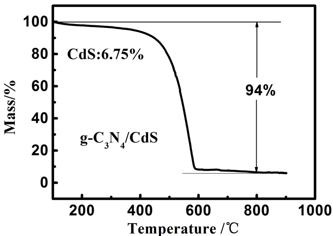
Fig. S1 Thermal gravimetric analysis (TGA) curves of the g-C 3 N 4 -CdS.
