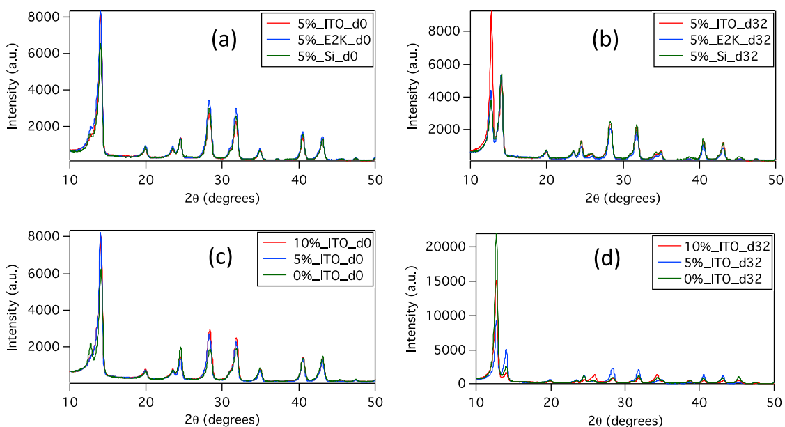
Fig. S1 GIXRD scans as a function of substrate and chlorine composition.
