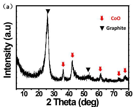
Figure S1. XRD patterns of the CoO NWAs.
