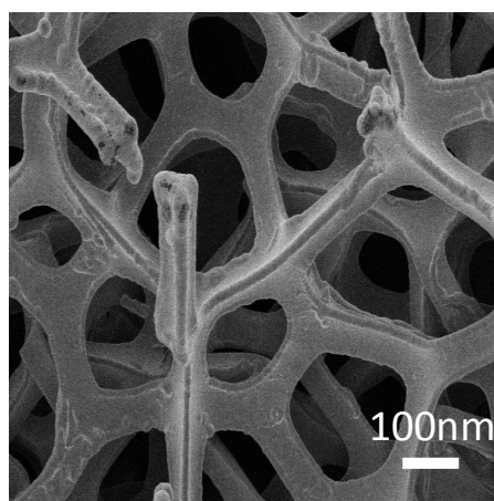
Figure S1. SEM image of bare Ni foam.
