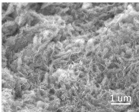
Figure S3. SEM image of CoS@NiCo 2 S 4 NWSAs after 3000 cycles.
